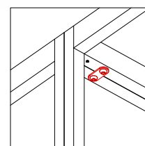
Linear joint plate
